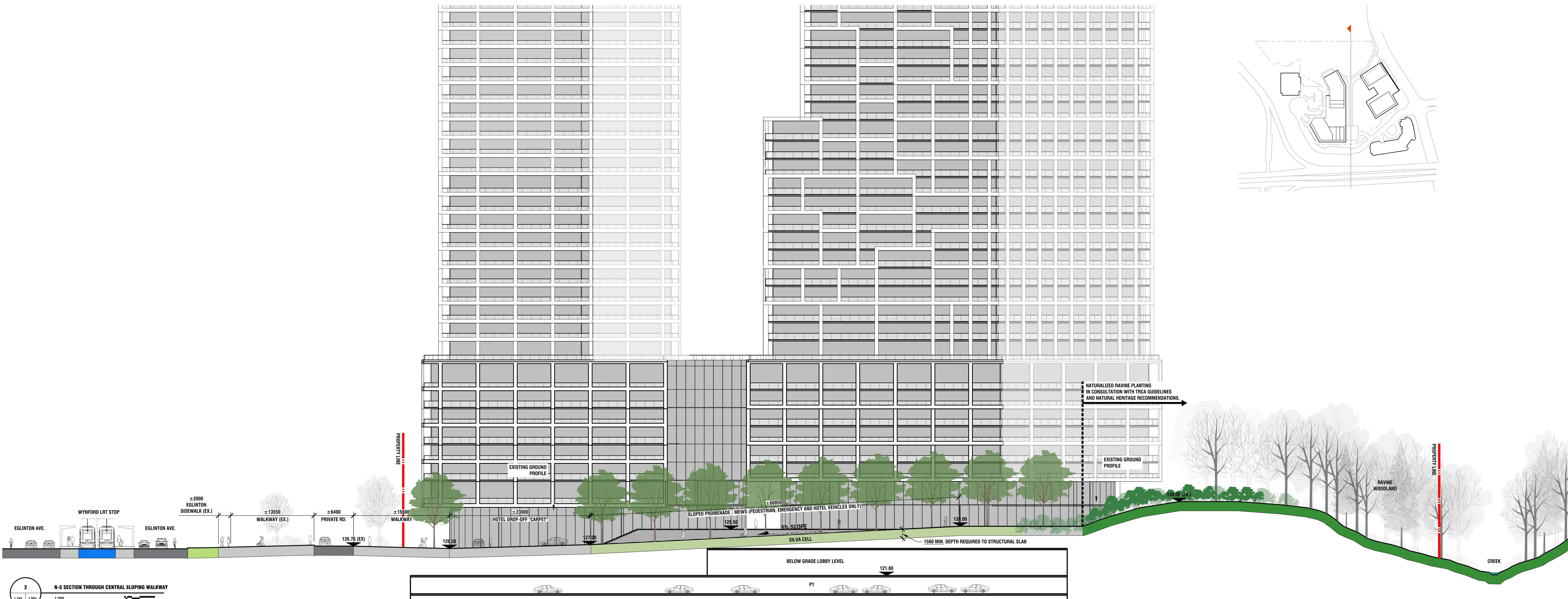
1 N-S SECTION THROUGH CENTRAL SLOPING LAWN 1:250
